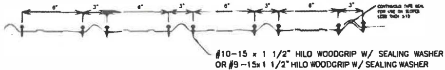
TYPE 2 FASTENER PATTERN AT 24" O.C.
