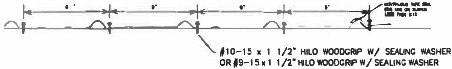
TYPE 2 FASTENER PATTERN AT 24" O.C.
