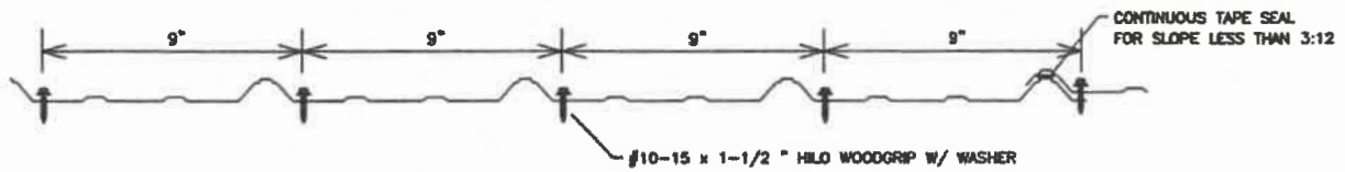
FASTENER PATTERN TYPE 1
